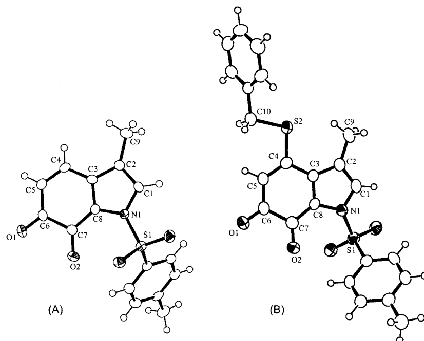
Figure 1. ORTEP drawings of compound 7 (A) and compound 8 (B) showing 50% probability thermal ellipsoids
