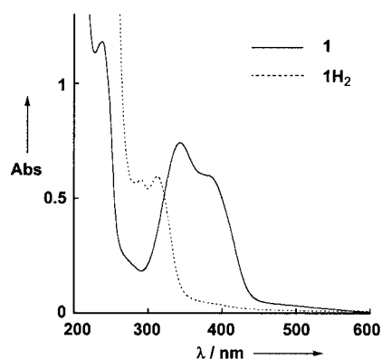
Figure 2. UV/Vis spectra of 1 ( 5.0 \times 10^{-5}\text{ M} ) and its quinol derivative 1H 2 , generated by the reduction of 1 with \text{MeNHNH}_2 (10 equiv.) in \text{CH}_3\text{CN}
